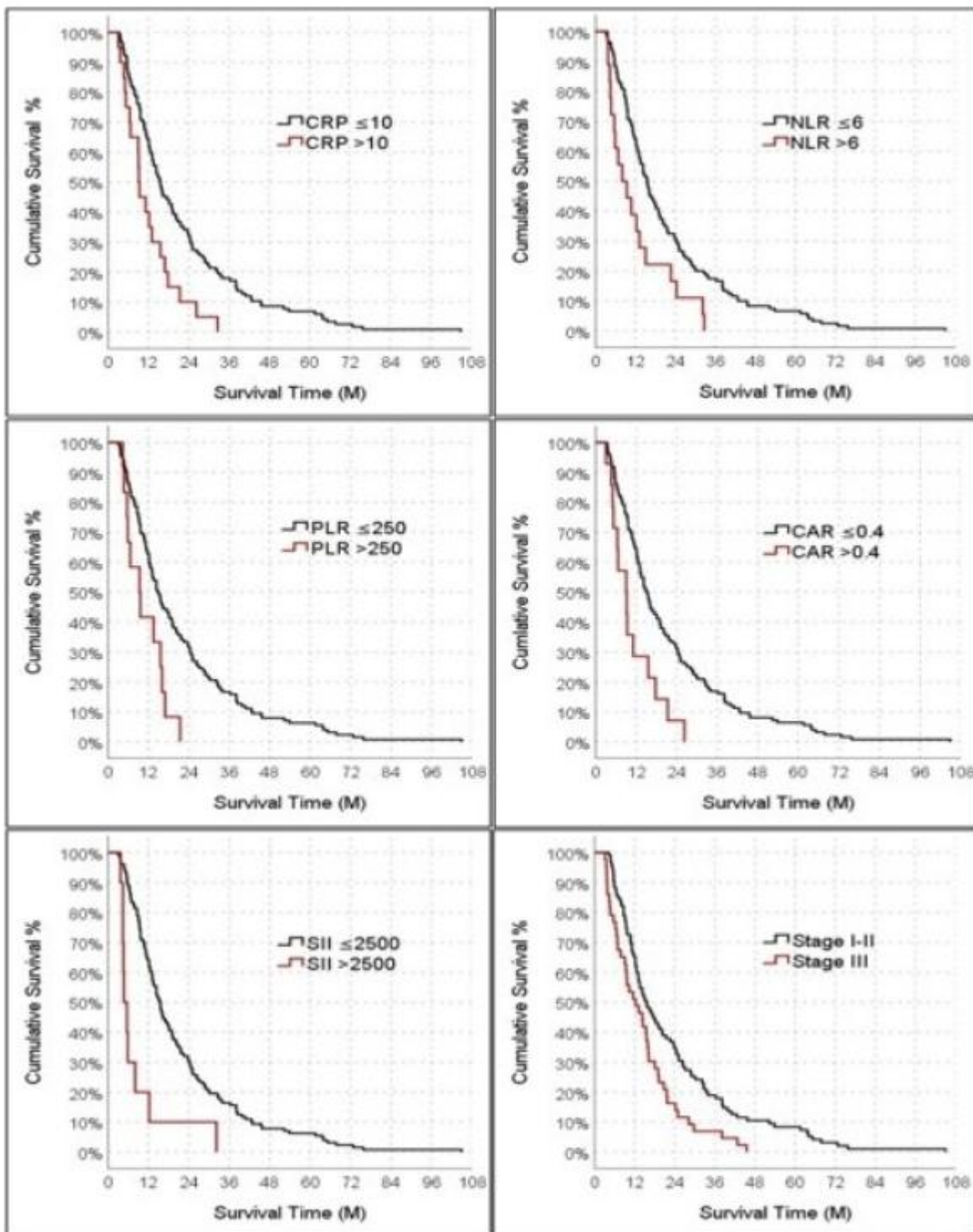
Figure 2. Kaplan–Meier survival curves according to hematologic indexes associated with overall survival (OS) when divided into 2 groups (high/low). OS outcomes according to indexes including CRP, NLR, PLR, CAR, SII and stage ( P < 0.05 ).
